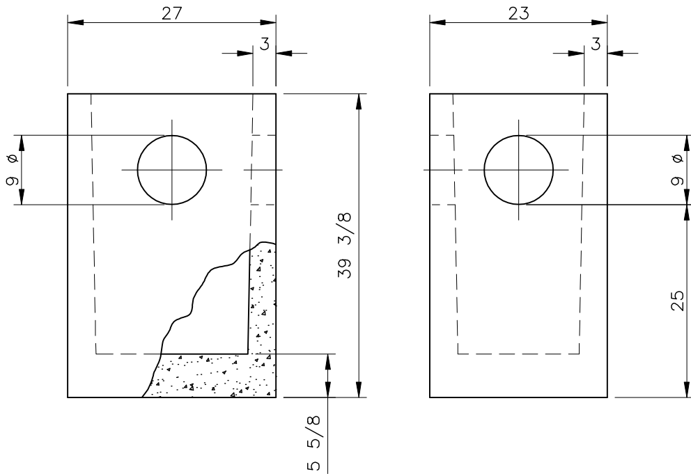
SIDE VIEWS
